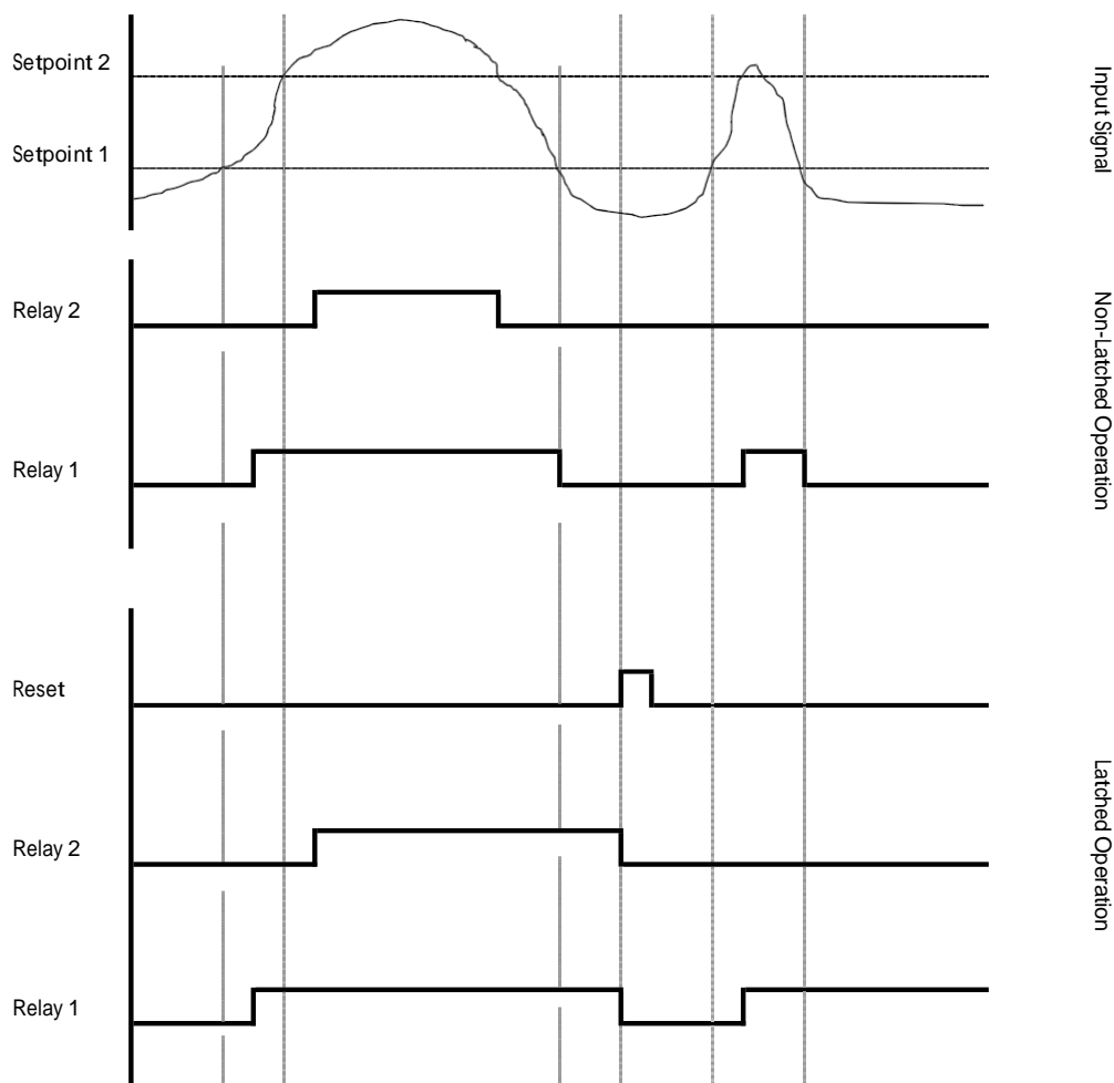
Figure 2: SI-509 Relay Non-Latching / Latching Principle of Operation
