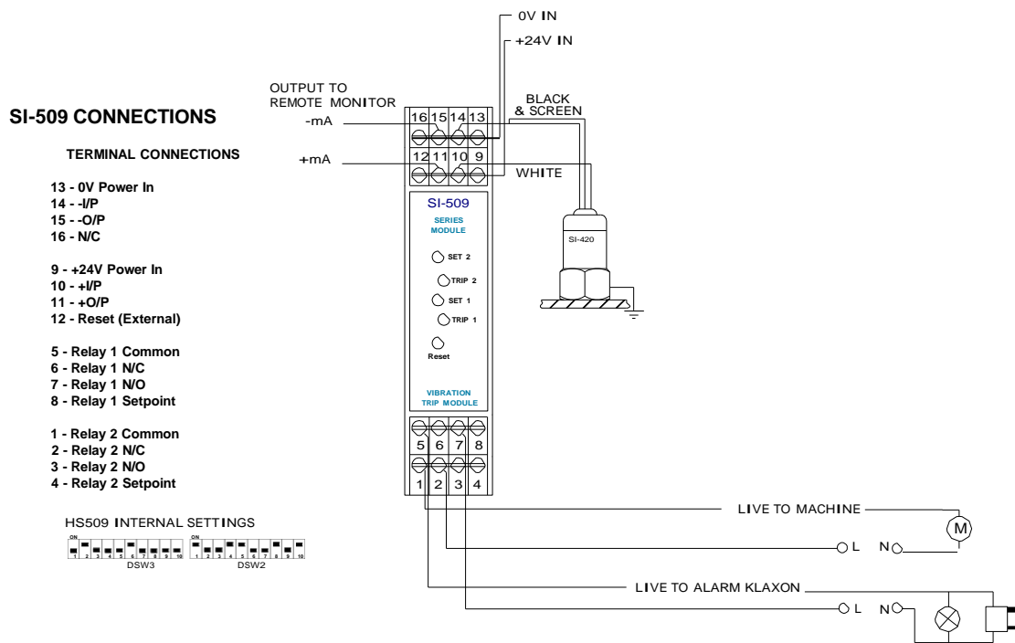
Figure 1: SI-509 Example Wiring Diagram
